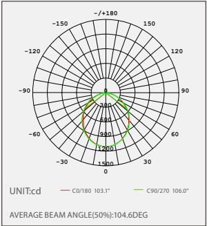
LUMINAIRE PHOTOMETRIC for 1.2M 6000K
