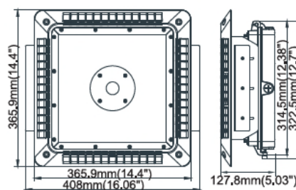
P2 Recessed Installation Frame
