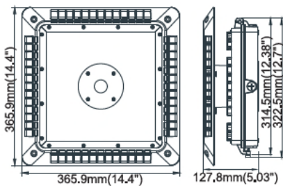
P1 Surface mounting installation (Standard)
