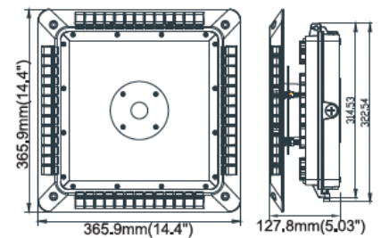
P3 American installation ways
