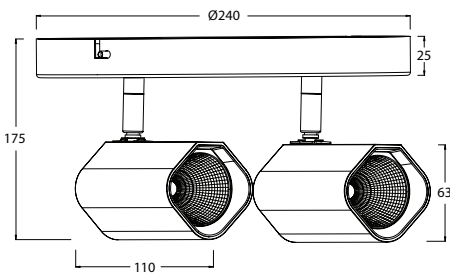
A-Double
