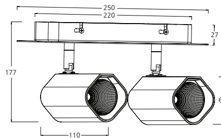
B-Double
