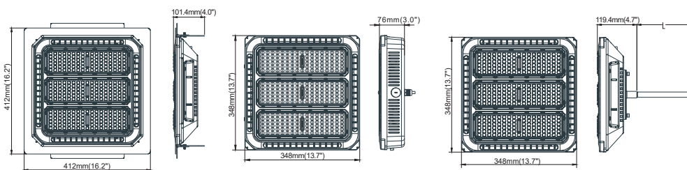
P1 Recessed Installation Frame (Standard)
