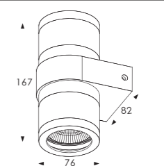
Painting color RAL9006 (White aluminium color)
