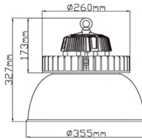
Aluminum reflector 90degree
