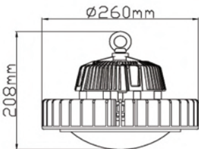
No reflector 120degree
