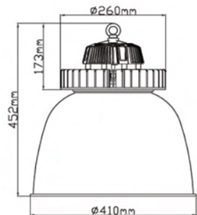
PC reflector 70degree
