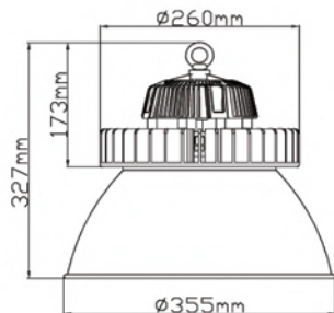
Aluminum reflector 60degree
