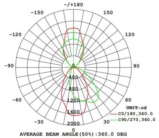
1.2m luminaire with Microprism
