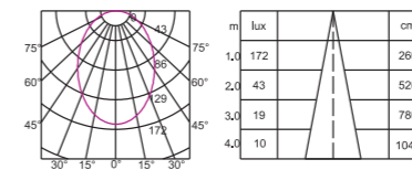
GKSML3007 7W 3000K CRI>90 110°
