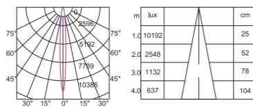
GKSMS5515 15W 3000K CRI>90 15°
