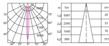
GKSMS5515 15W 4000K CRI>90 15°
