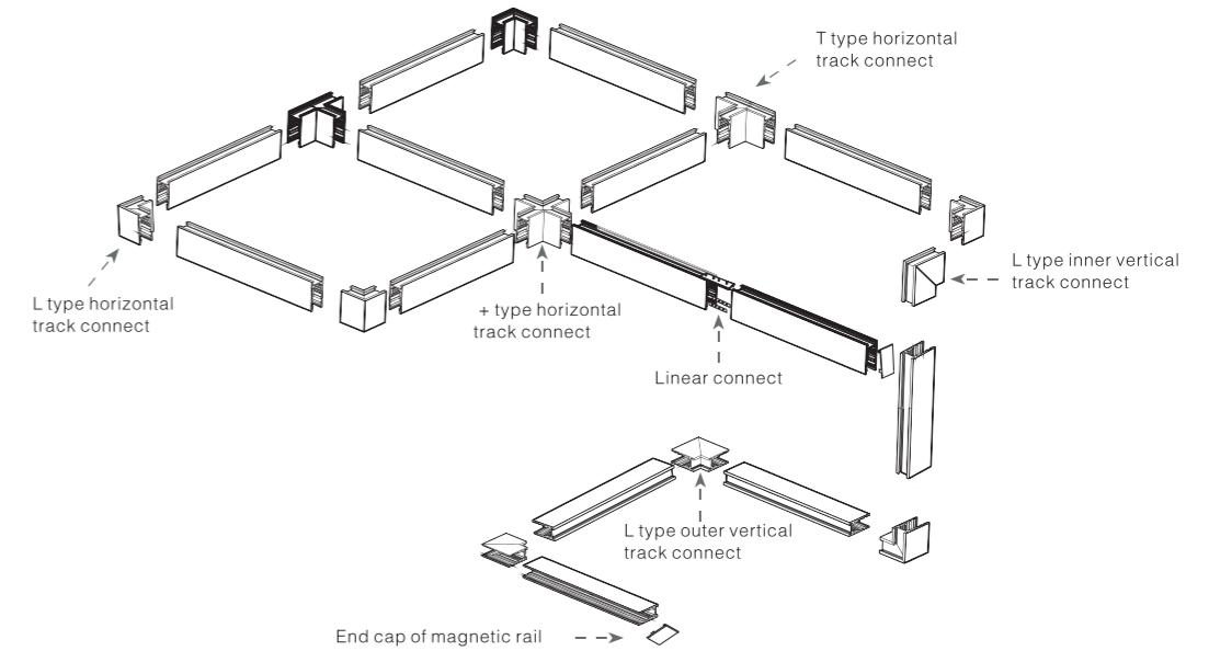
Rail connection of recessed installation
