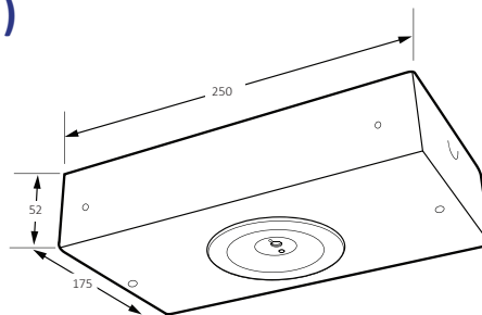
Surface ceiling mounting 250*175*52mm
