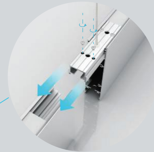
GLH25 Connection (without end cap)
