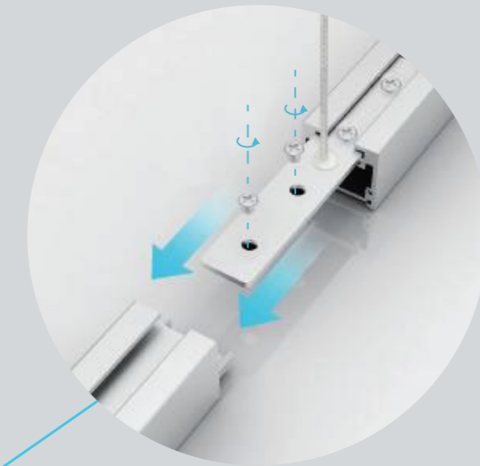
GLS25/GLM25/ GLE25/GLR25 Connection (without end cap)
